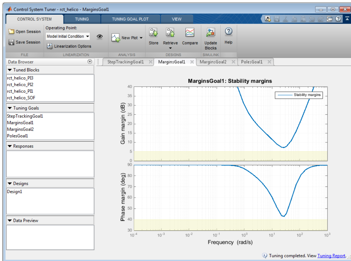
Figure 15: Control System Tuner App with Stored Design1.
