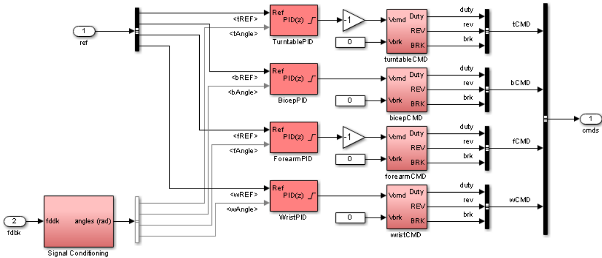
Figure 2: Controller structure.
