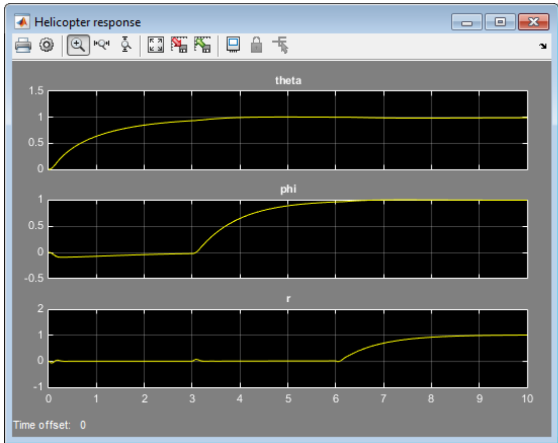
Figure 17: Nonlinear Response of Tuned PI controllers.
