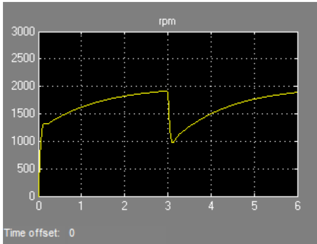
Figure 20: Nonlinear Simulation of Tuned Controller.
