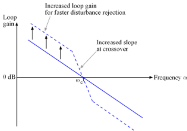
Figure 1: Trade-off in 1-DOF PID Tuning.
