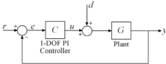
Figure 2: PI Control Loop.
