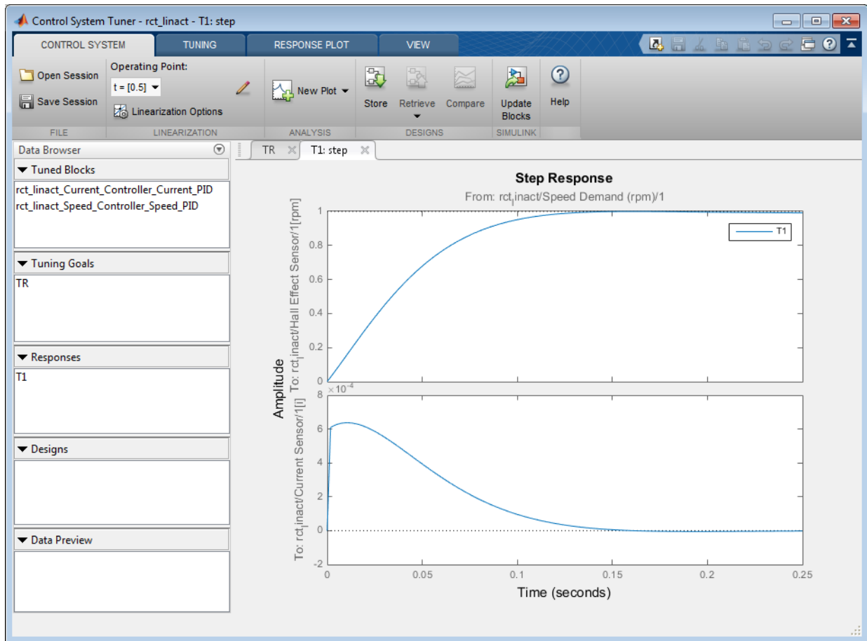
Figure 18: Step Plot in Control System Tuner App.
