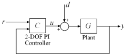
Figure 3: 2-DOF PI Control Loop.
