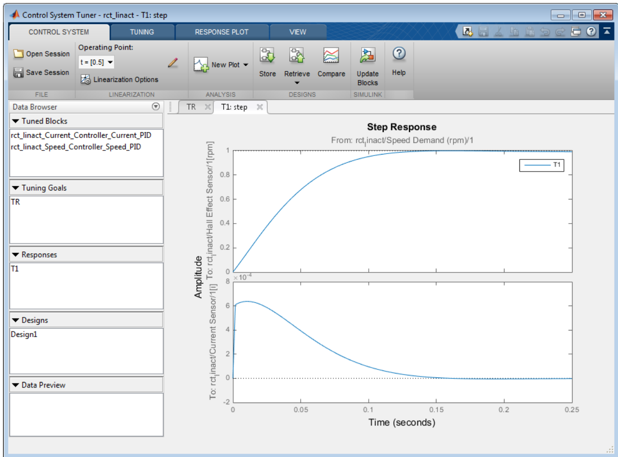
Figure 19: Stored Values of Tuned Blocks in Control System Tuner App.
