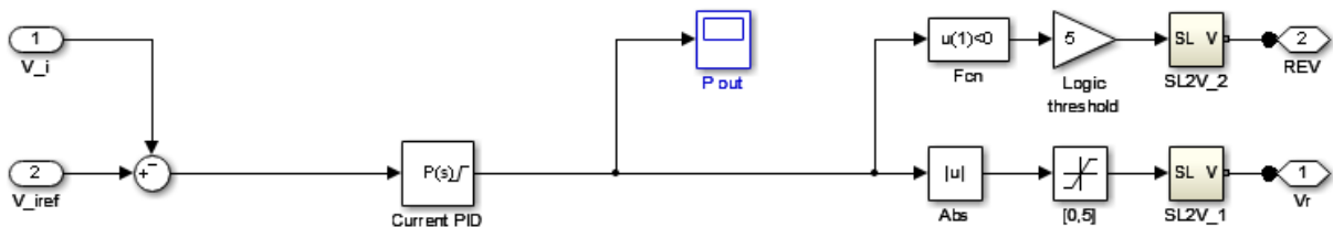
Current Controller
