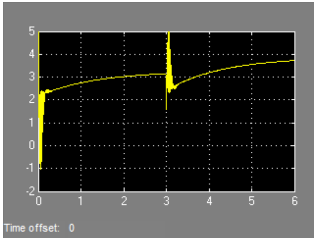
Figure 21: Current Controller Output (limited to plus/minus 5).
