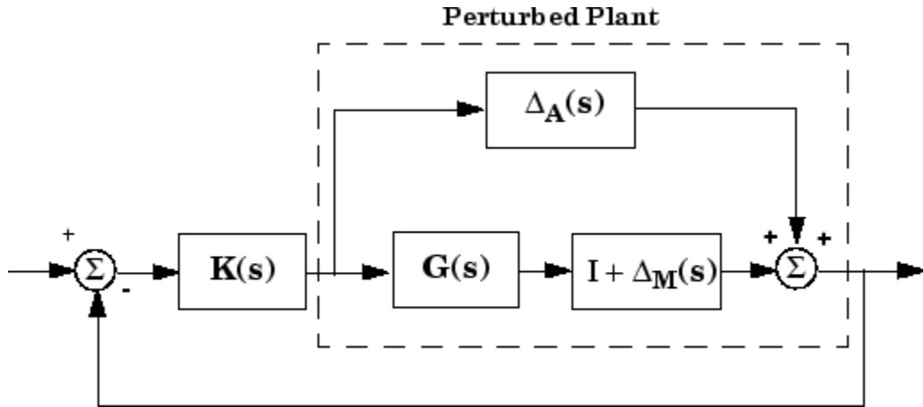
Additive/Multiplicative Uncertainty
