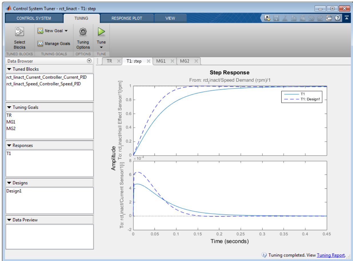
Figure 27: Step Responses of Two Designs.
