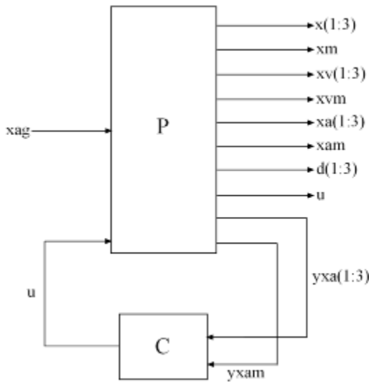
Figure 2: Control Structure
