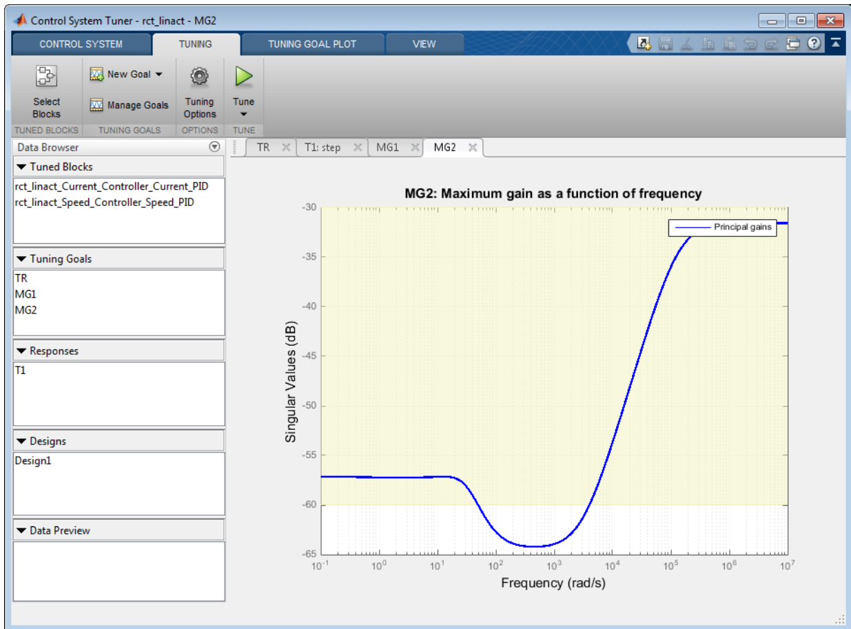
Figure 24: Two Gain Goals Added to Control System Tuner App.
