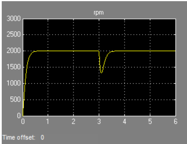
Figure 28: Nonlinear Response of Tuning with Gain Constraints.
