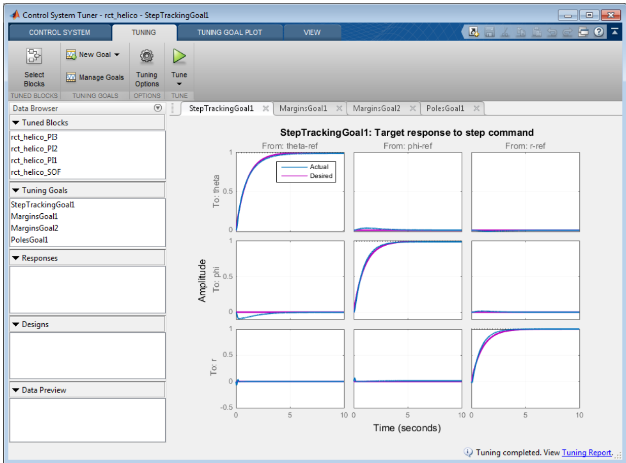
Figure 13: Control System Tuner App After Tuning.
